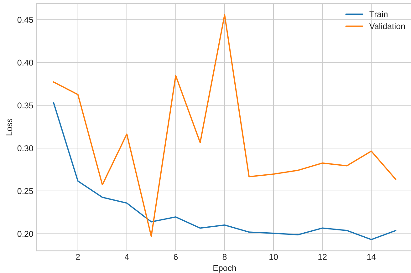
PNEUMONIA vs NORMAL Loss
