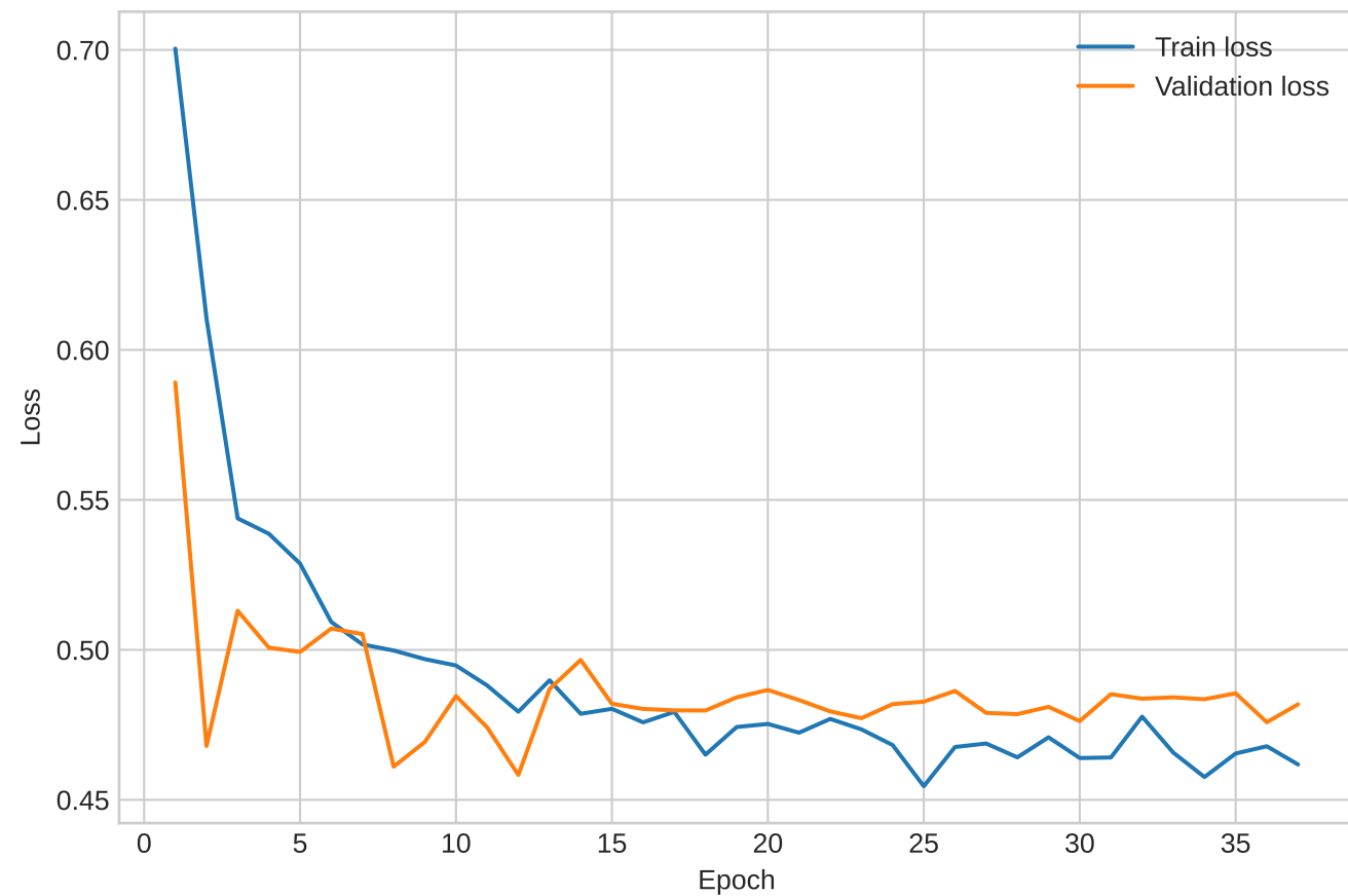
Task 2 DenseNet121 Loss
