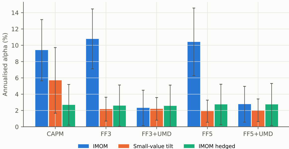
Alpha shrinks as known factors are added (95% Newey-West CI)
