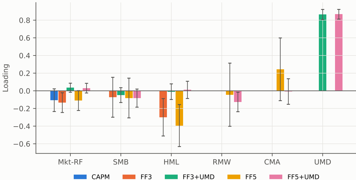
Industry momentum factor loadings by model (95% Newey-West CI)
