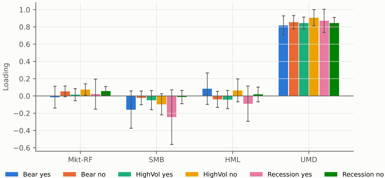
Industry momentum exposures by regime (FF3+UMD, 95% NW CI)
