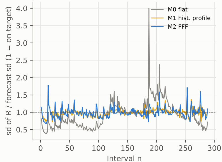
EUR/USD: realised risk / target, test
