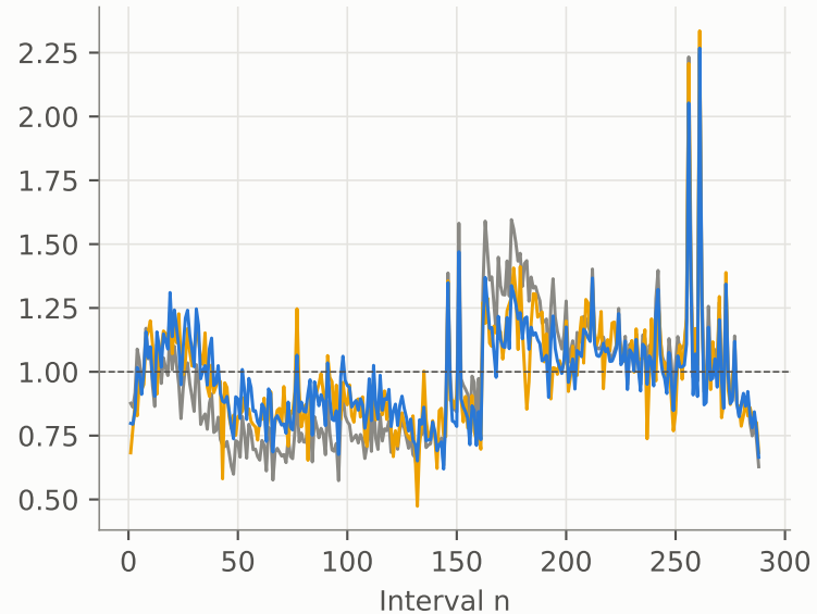
BTC/USDT: realised risk / target, test
