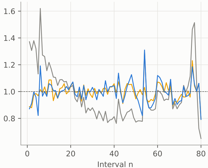
S&P 500: realised risk / target, test
