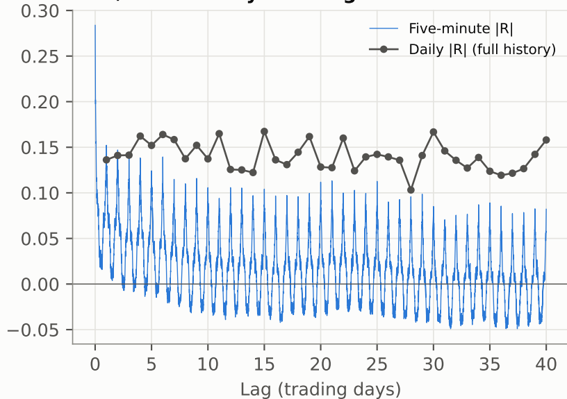
EUR/USD: 40-day correlogram
