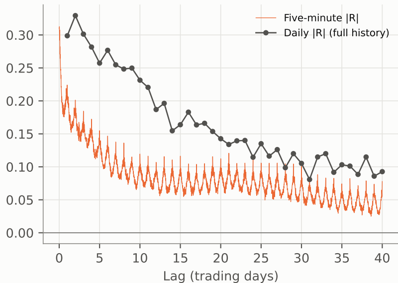
S&P 500: 40-day correlogram
