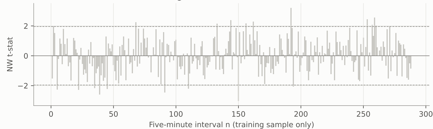
BTC/USDT: 0 of 288 intervals significant after FDR control (21 at naive 5%)
