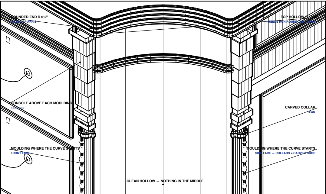
CORNER CLOSE-UP FRONT RIGHT · HOLLOW, ROUNDS, END MOULDINGS, CONSOLES
