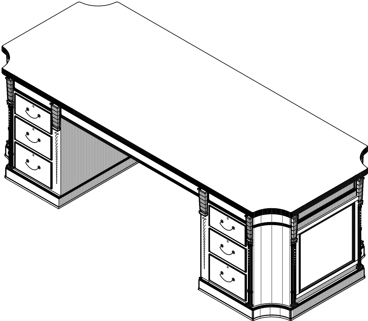
FROM THE FRONT RIGHT AXONOMETRIC · HIDDEN LINES REMOVED · SHADED
