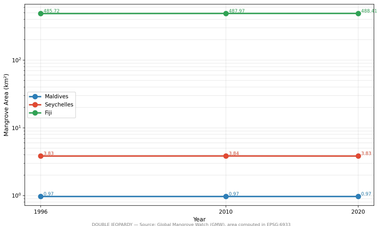
Figure 3. Mangrove extent (km², log scale) at three independent time points (1996, 2010, 2020) for the three islands where mangroves are present. Extent remains essentially flat for all three islands, with no measurable decline detected.
