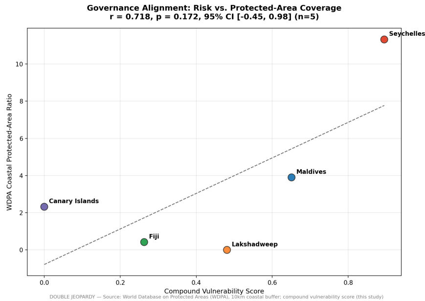
Figure 6. Compound Vulnerability Score plotted against the coastal WDP coastal protected-area ratio for each island, with a fitted OLS reference line. r = 0.718 , p = 0.172 , 95% CI [-0.45, 0.98] (n=5) — a positive but statistically inconclusive relationship, driven by the small sample size rather than a null result.
