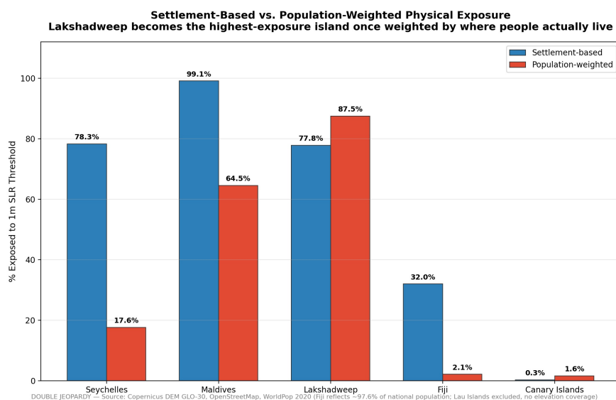
Figure 2. Settlement-based versus population-weighted physical exposure by island. Lakshadweep becomes the highest-exposure island once weighted by where population is actually concentrated,
