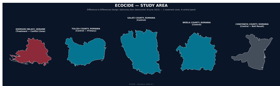
Figure 1. Study area showing the treatment zone (Kherson Oblast, Ukraine) and the four-county control panel used in this study — Tulcea, Galați, Brăila, and Constanța, Romania. Administrative boundaries were obtained from GADM v4.1. The control counties were selected to represent comparable river-delta, steppe, and coastal ecosystems along the Danube/Black Sea corridor while remaining unaffected by the Kakhovka Dam destruction, enabling causal estimation through matched treatment-control comparison.
