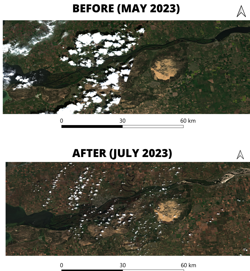
Figure 2. Sentinel-2 true-colour imagery of the Kakhovka reservoir immediately before (May 2023) and after (July 2023) the destruction of the Kakhovka Dam. The post-event image reveals the near-complete drainage of the reservoir and extensive exposure of the former lakebed. This pair is presented to illustrate the spatial scale of the event and to motivate the statistical analysis that follows; it is not, on its own, evidence of a causal effect — that evidence is established
