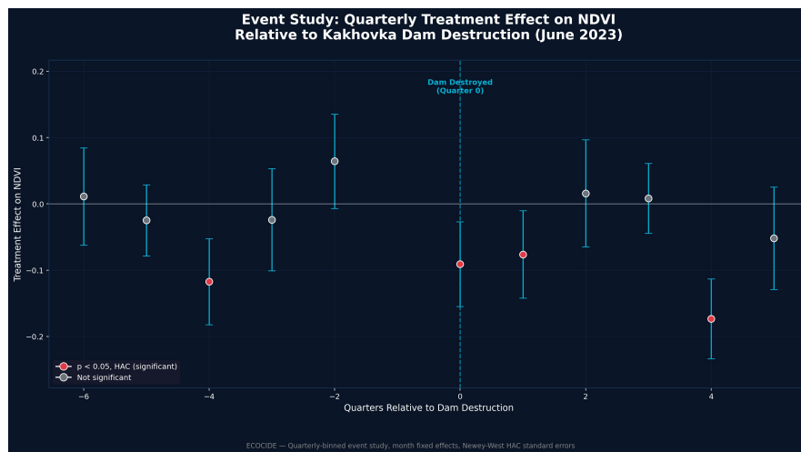
Figure 6. Quarterly event-study estimates (Newey-West HAC standard errors) showing treatment effects relative to the pre-event baseline. Significant negative effects emerge during the treatment quarter, the following quarter, and one year later, while a statistically significant pre-treatment coefficient highlights the influence of earlier conflict-related vegetation changes in Kherson. This pre-treatment signal motivated the sensitivity analysis and is reported transparently as a methodological limitation rather than being excluded.
