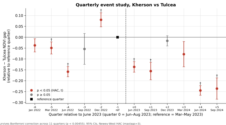
Figure 6. Quarterly event study of the Kherson-Tulcea NDVI gap; 95% HAC confidence intervals; † survives Bonferroni correction.
