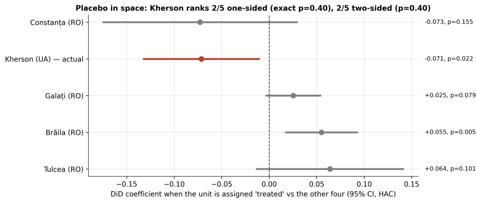
Figure 8. Placebo in space: each unit assigned “treated” status against the other four.
