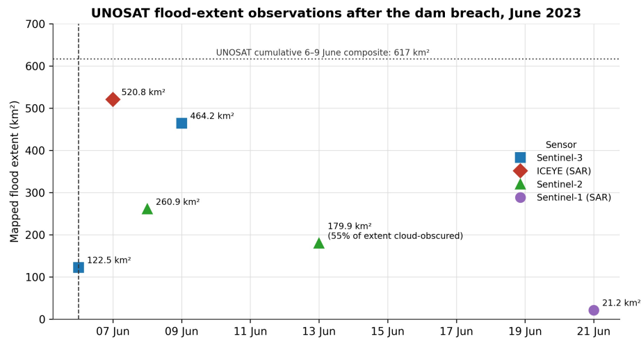
Figure 3. Flood extent in each UNOSAT layer, by sensor. Points are separate observations.
