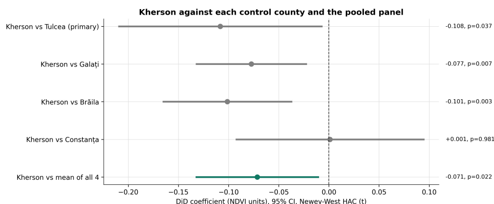
Figure 7. Kherson against each control county and the four-county mean; 95% HAC confidence intervals.
