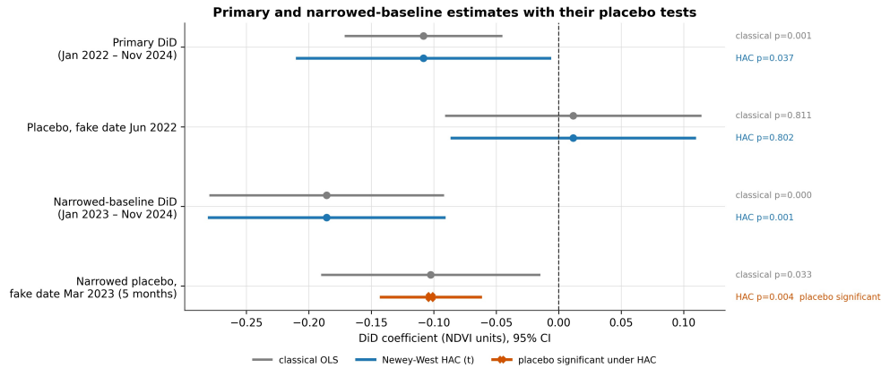
Figure 5. Primary and narrowed-baseline estimates with their placebo tests; classical and HAC 95% confidence intervals.
