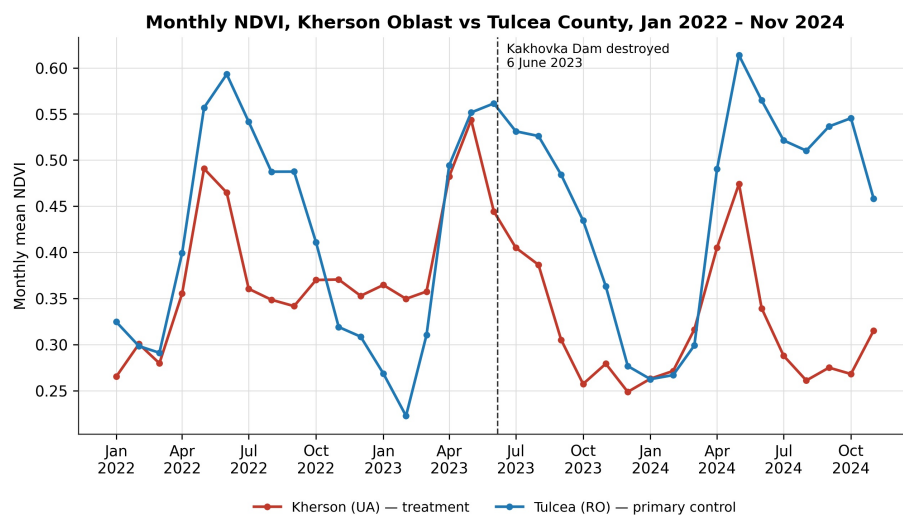
Figure 4. Monthly mean NDVI, Kherson Oblast and Tulcea County (cloud- and water-masked monthly median composites).
