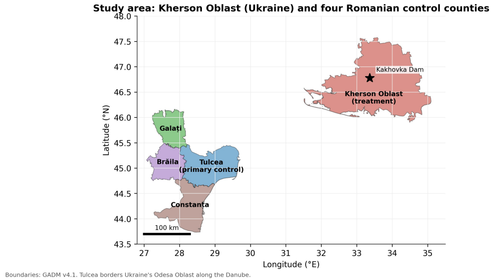
Figure 1. Treatment zone and the four Romanian control counties (GADM v4.1). Star: Kakhovka Dam.
