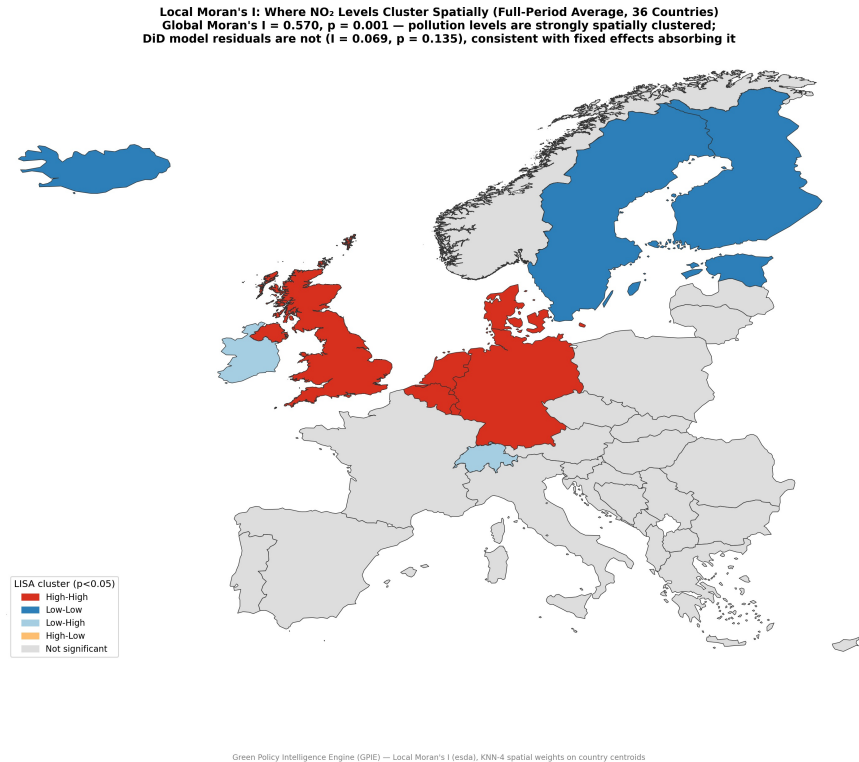
Figure 9. Local Moran's I (LISA) clusters for full-period average NO 2 , across all 36 countries in the panel. Red marks the High-High cluster (Benelux/Northern industrial corridor plus the UK), blue marks the Low-Low cluster (Nordic/Baltic plus Iceland), light blue marks significant Low-High outliers (Switzerland, Ireland).
