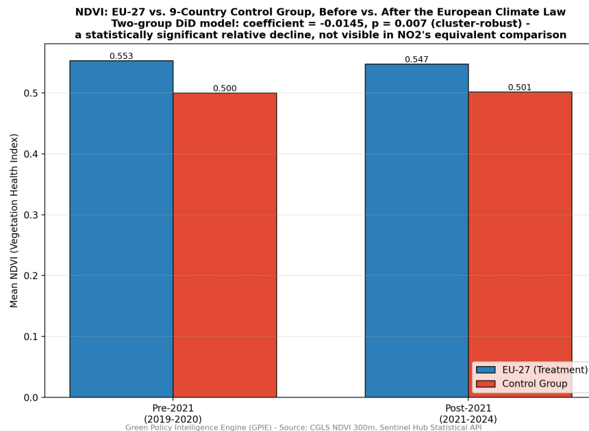
Figure 4. Mean NDVI for the EU-27 treatment group and the non-EU control group, before (2019-2020) and after (2021-2024) the European Climate Law. Unlike the equivalent NO 2 comparison (Figure 2), the two groups’ NDVI trajectories diverge — the visual basis for the significant relative decline reported above.
