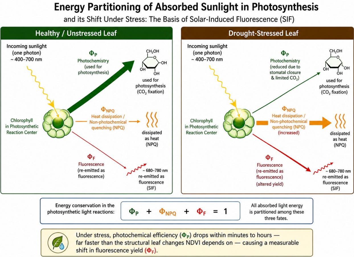
Figure 1. Schematic representation of leaf-level light energy partitioning among photochemistry, non-photochemical quenching (heat dissipation), and chlorophyll fluorescence, under well-watered versus drought-stressed conditions.
