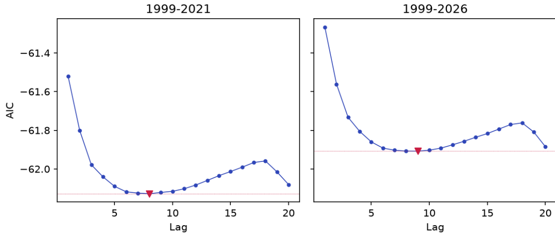
Figure 13: Lag Selection Diagnostics
