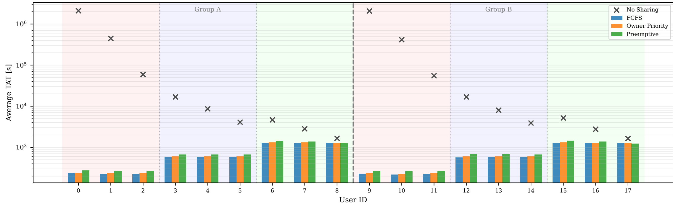
Per-user Average TAT (system load \approx 0.5 )
