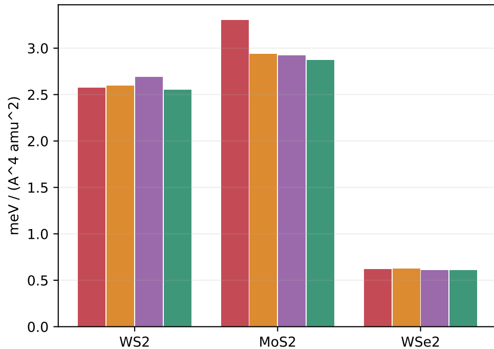
Signed quartic MAE vs PBE
