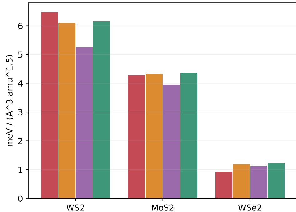
Cubic MAE vs PBE
