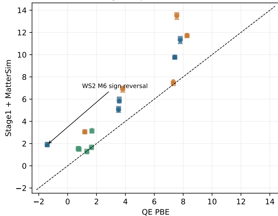
Signed quartic \Phi_{1122}
