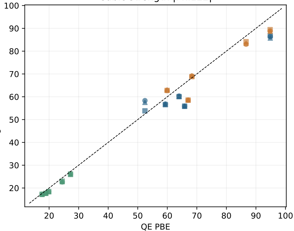
Cubic strength |\Phi_{122}|
