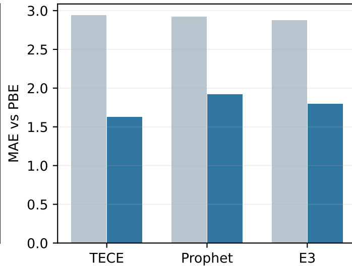
MoS2 / quartic
