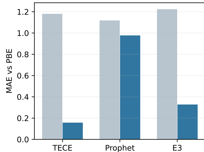
WSe2 / quartic
