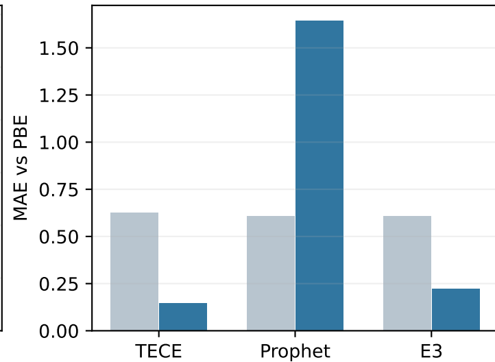
WSe2 / quartic
