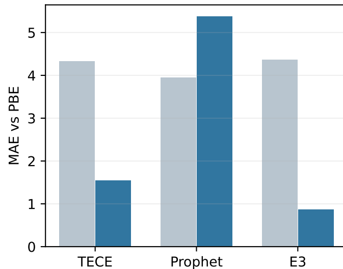
MoS2 / quartic
