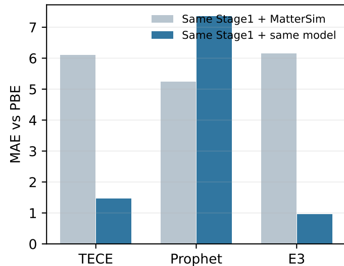
WS2 / quartic
