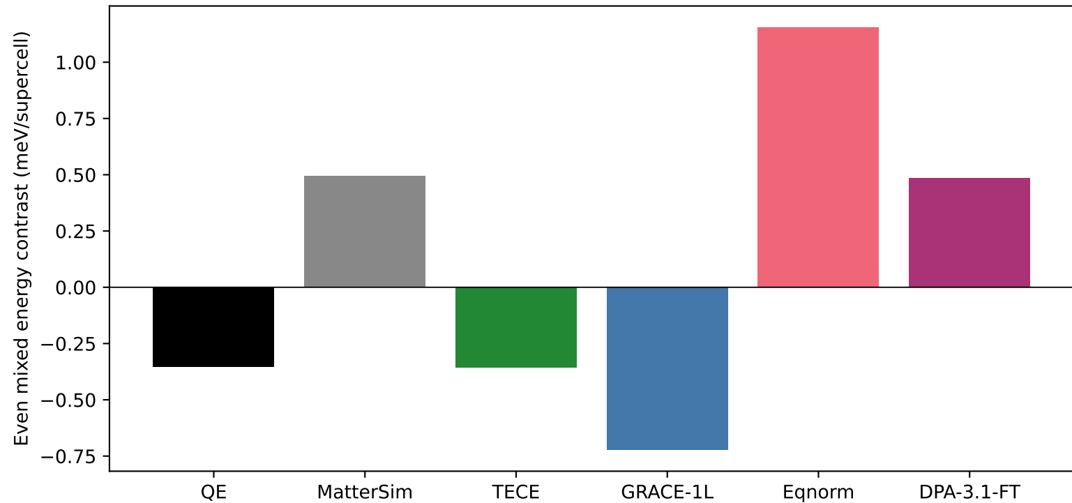
WS2 \Gamma 8-M6; identical PBE inputs, Q = 1
