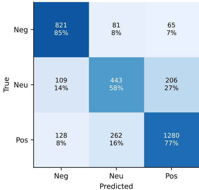
Train
