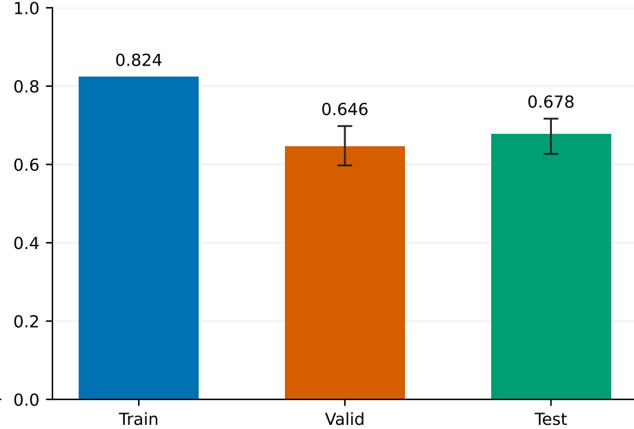
Pearson r
