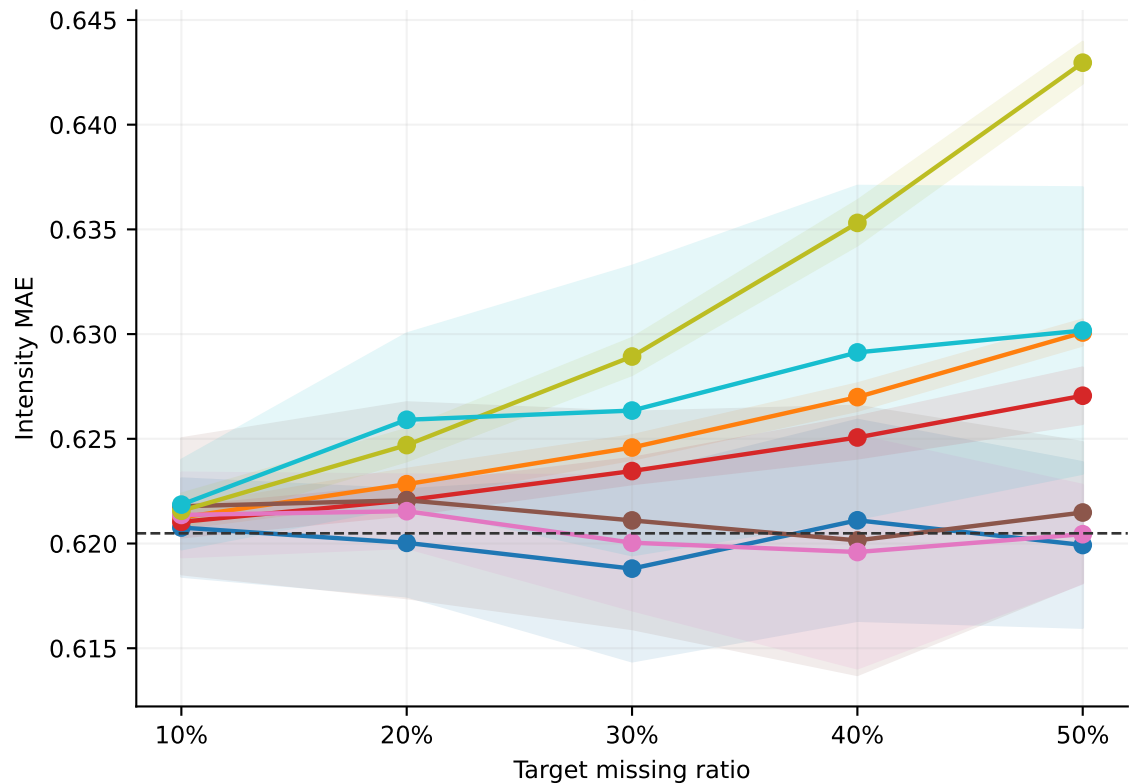
Intensity MAE
