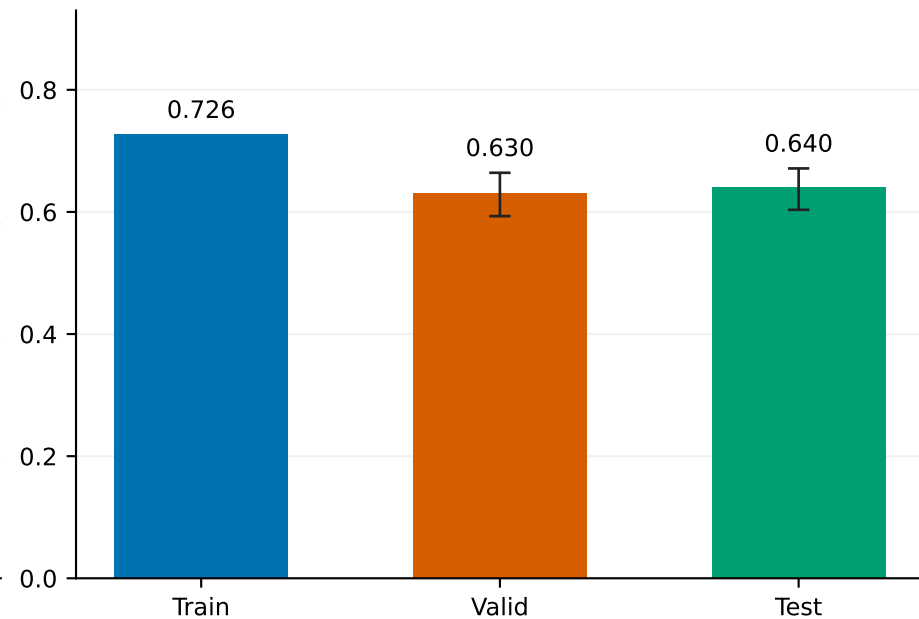
Pearson r
