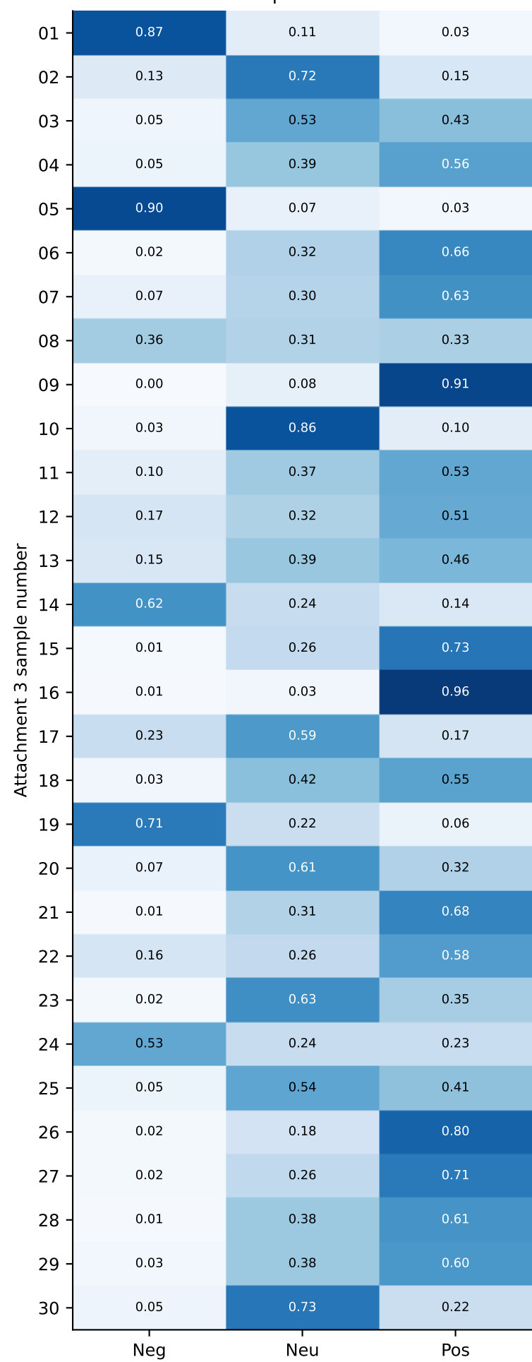
Class probabilities
