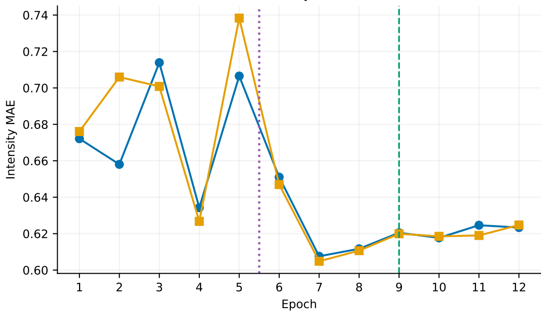
Intensity MAE
