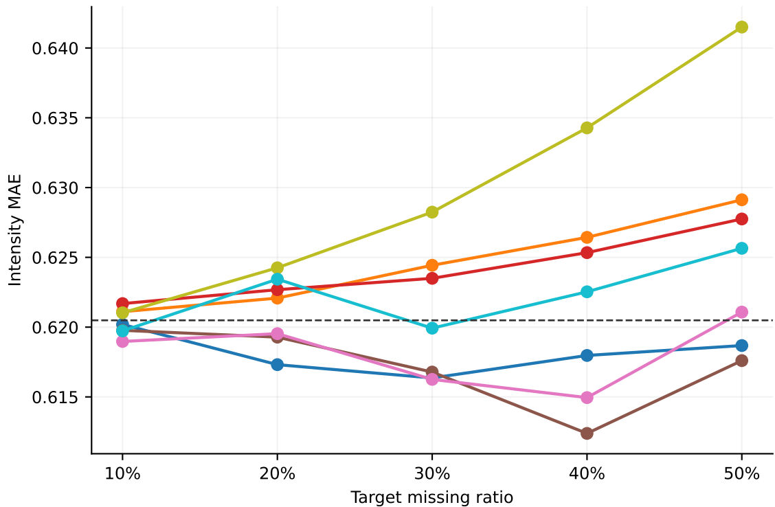
Intensity MAE
