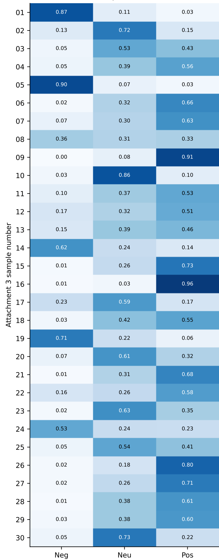
Class probabilities
