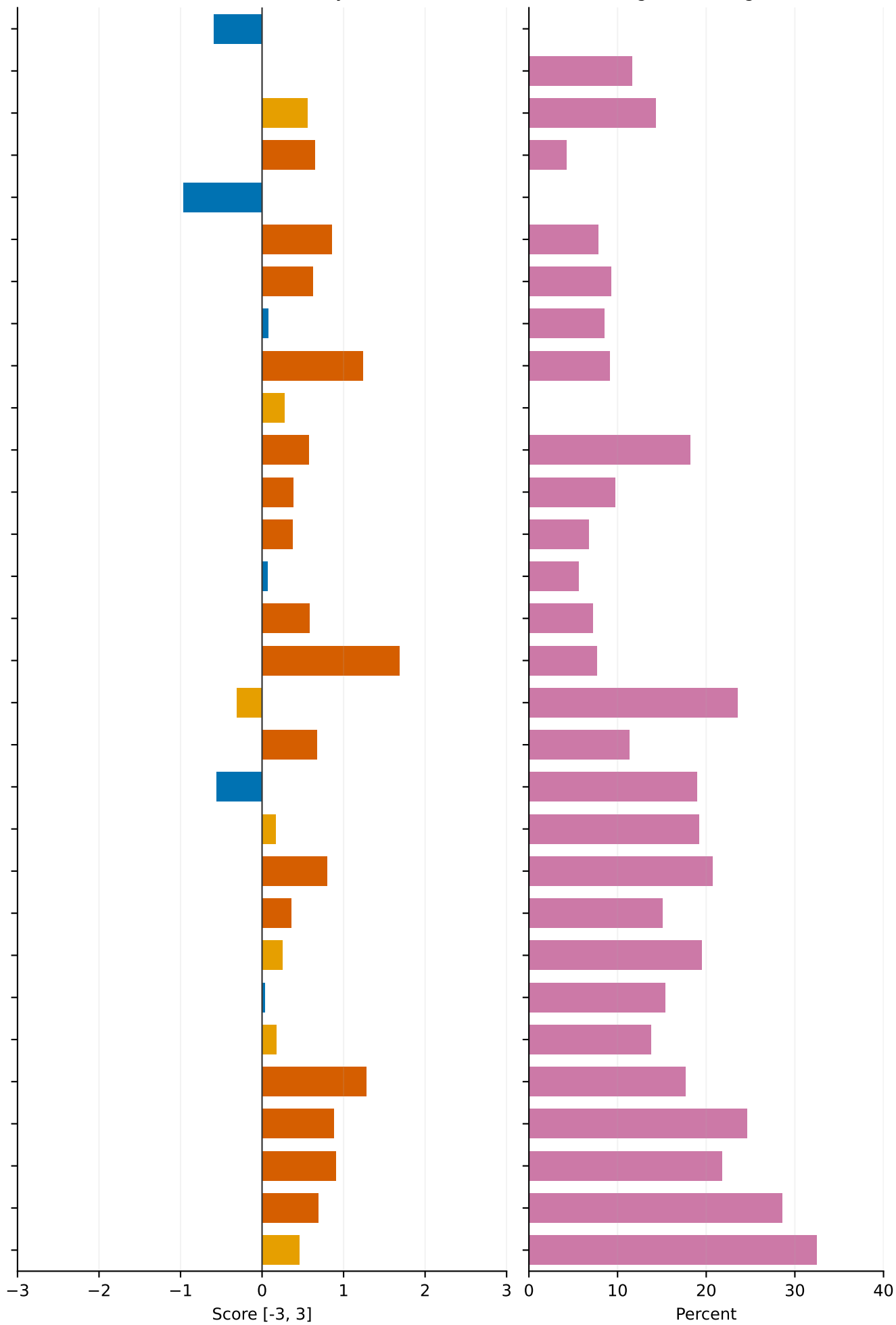
Predicted intensity
