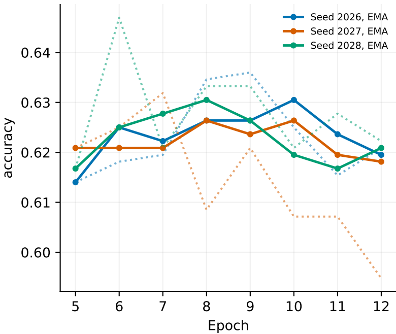
Validation accuracy
