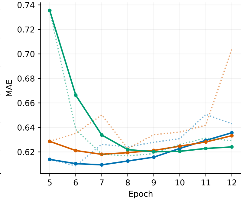
Validation MAE
