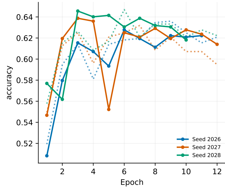
Validation accuracy
