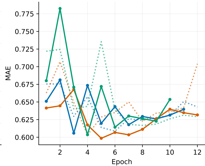
Validation MAE
