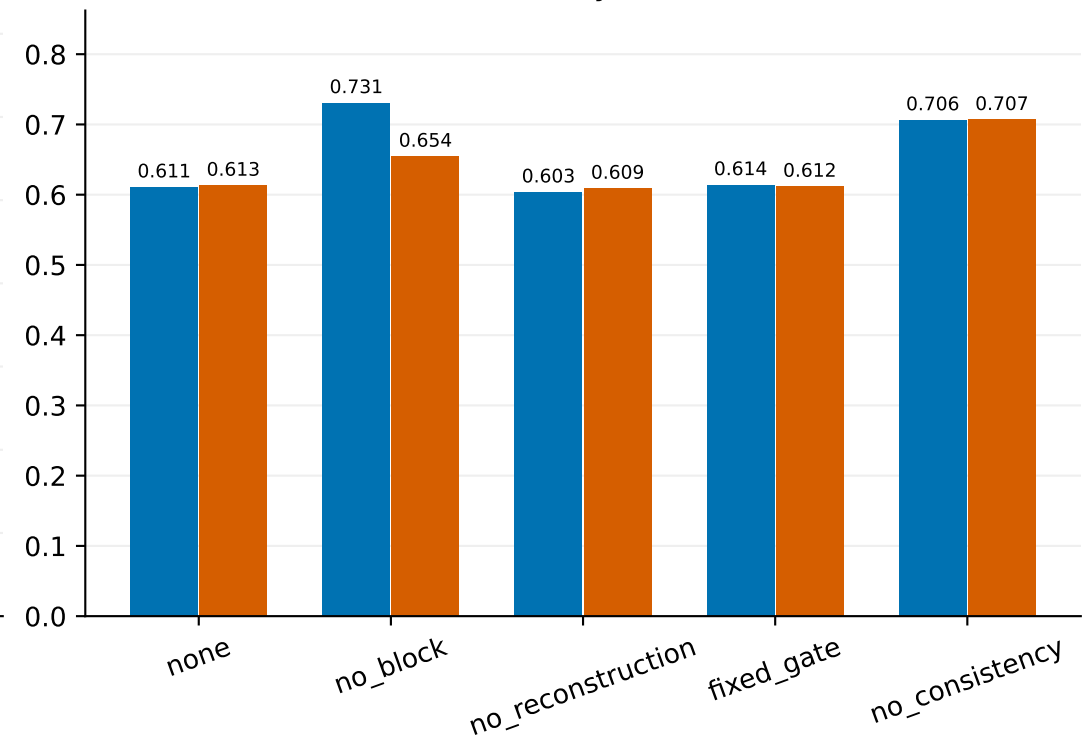
Intensity MAE
