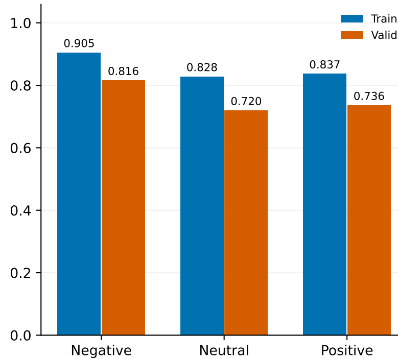
Accuracy (one vs rest)
