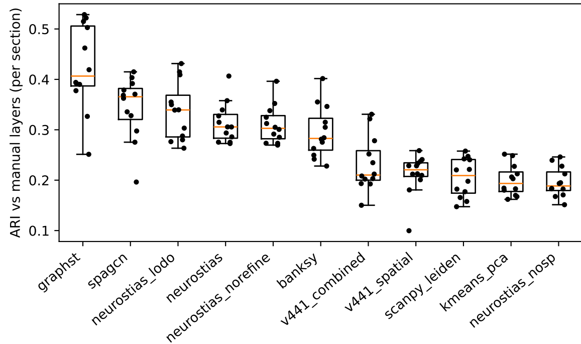
E01 DLPFC layer recovery (12 sections, mean of seeds)
