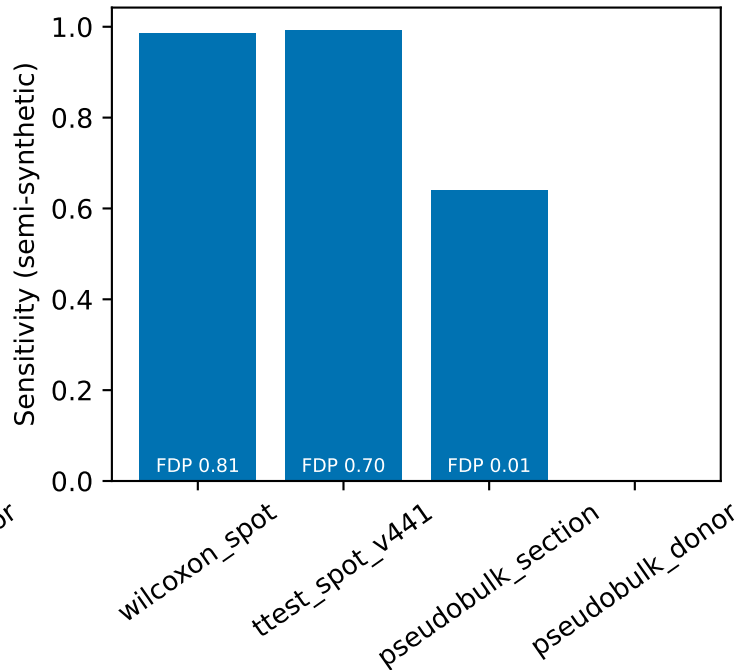
Known log2FC=1 in 200 genes
