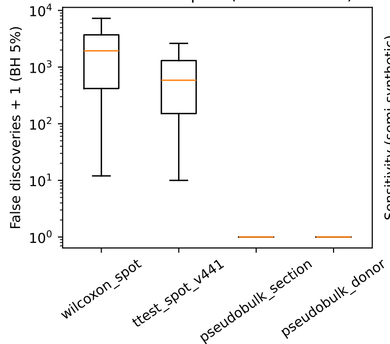
Null section splits (no true effect)
