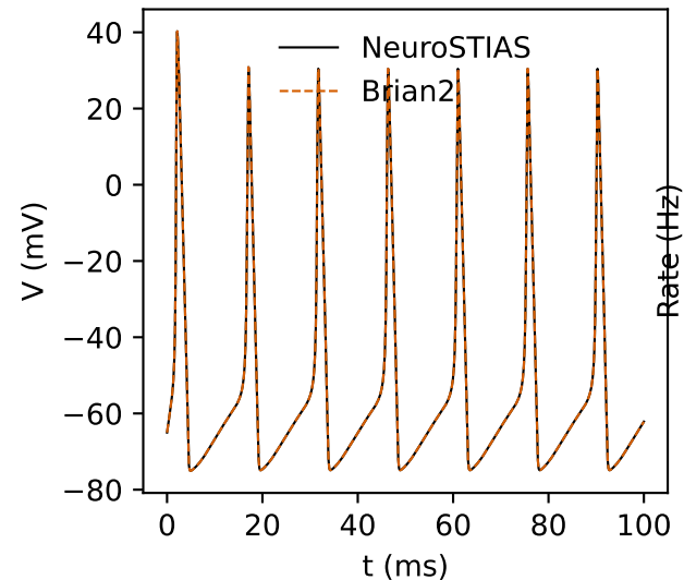
HH, 10 \mu\text{A}/\text{cm}^2
