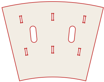
SEAT-DECK-2 x1
