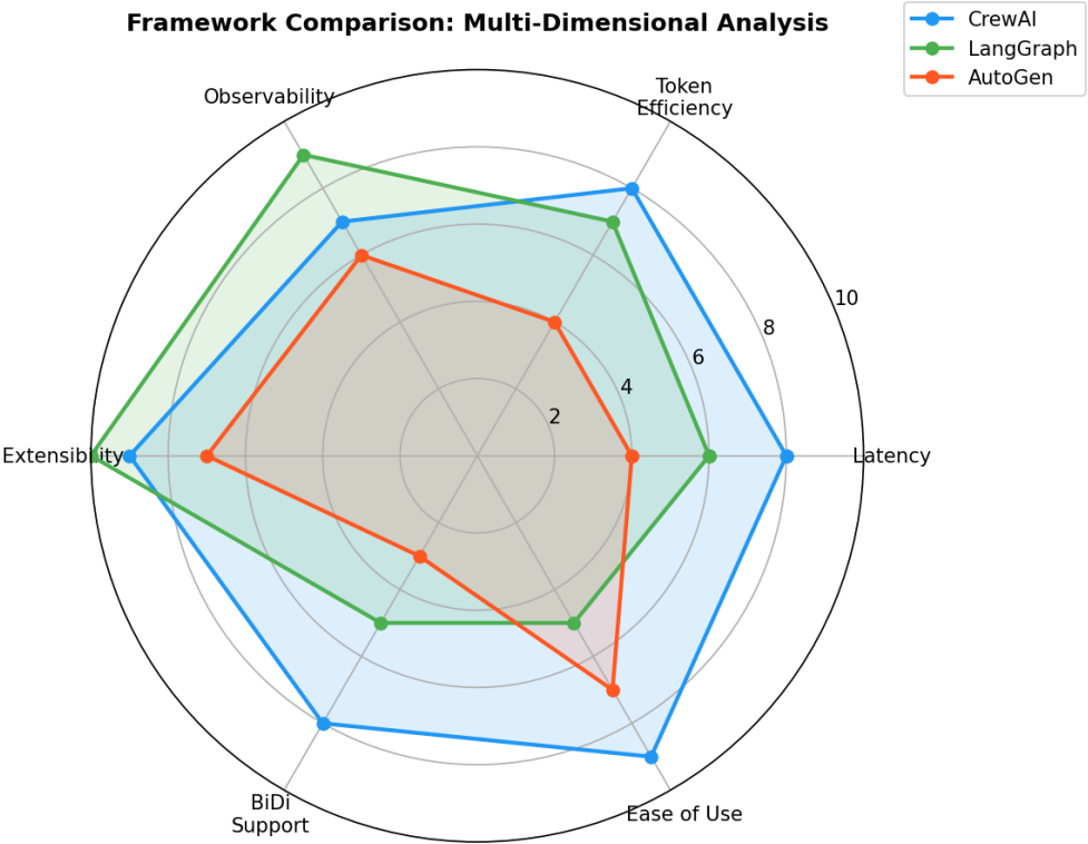
Figure 3.1: Multi-dimensional framework comparison across six production-readiness criteria (scores 0–10). Latency is inverted: a higher score means lower latency. Scores reflect the analysis in §3.2–3.6.
