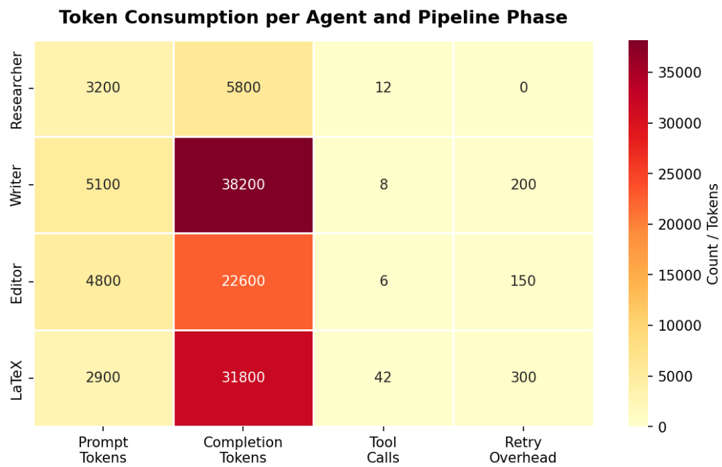
Figure 4.1: Token consumption heatmap across the four pipeline agents and four cost dimensions. Warmer colours indicate higher token usage; the Writer agent dominates completion tokens due to generating full chapter prose.
