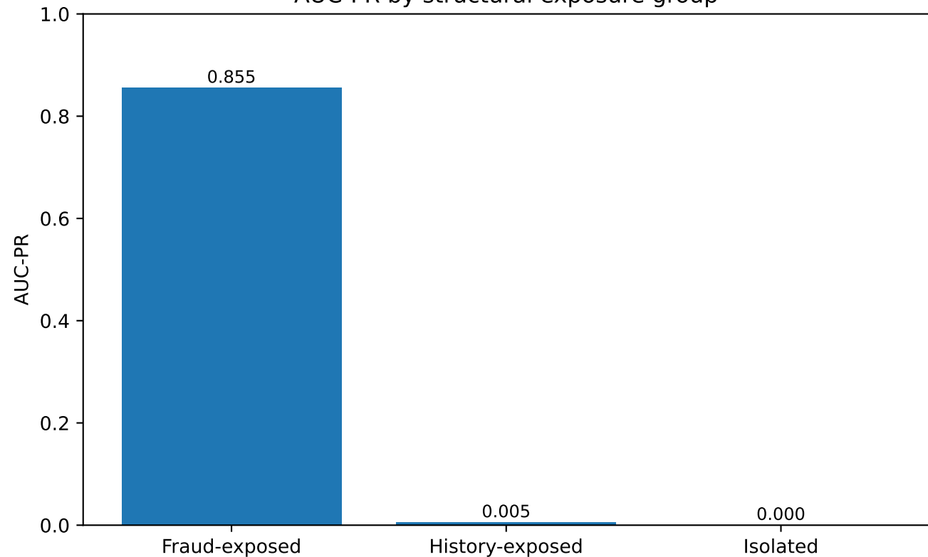
AUC-PR by structural exposure group
