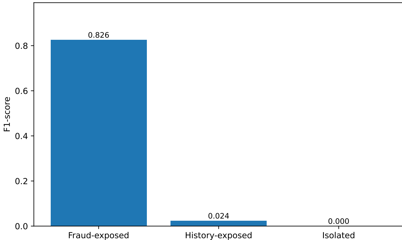
F1-score by structural exposure group
