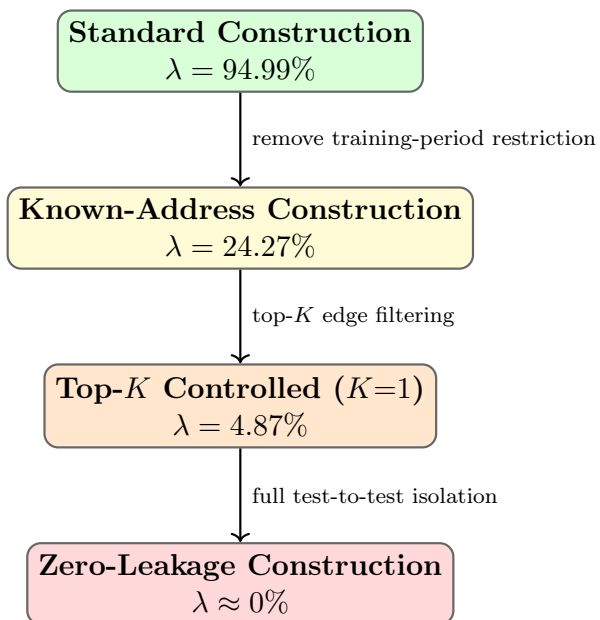
Figure 1: Connectivity spectrum used for leakage-aware evaluation. Test-to-test leakage \lambda is progressively reduced from 94.99% to near-zero through four graph-construction configurations, enabling quantification of the effect of structural connectivity on GNN performance.
