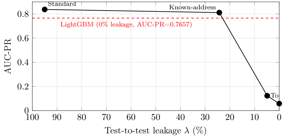
Figure 1: Impact of test-to-test leakage \lambda on GriffinGNN performance (solid line). AUC-PR remains at or above the LightGBM baseline (dashed red line) for \lambda \geq 24.27\% , but collapses well below it once \lambda \leq 4.87\% .
