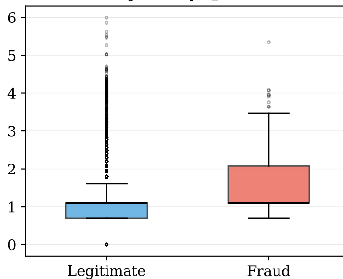
\log(1 + \text{burst\_activity})
