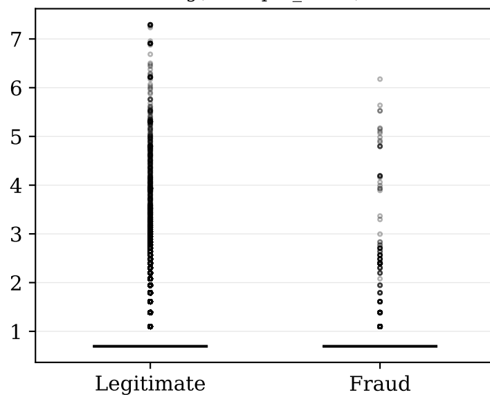
\log(1 + \text{address\_reuse\_count})
