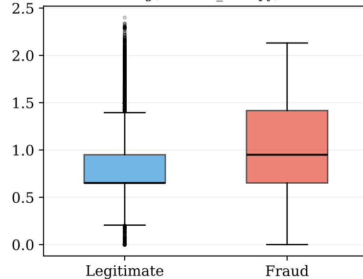
\log(1 + \text{graph\_metric})
