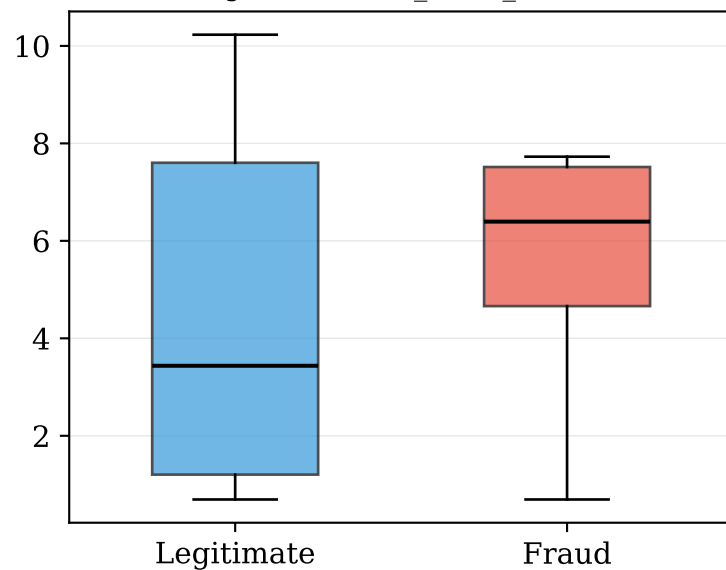
\log(1 + \text{address\_reuse\_count})
