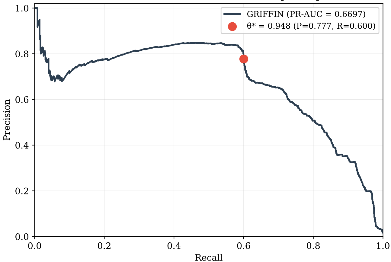
Precision-Recall Curve — GRIFFIN (Temporal Split)
