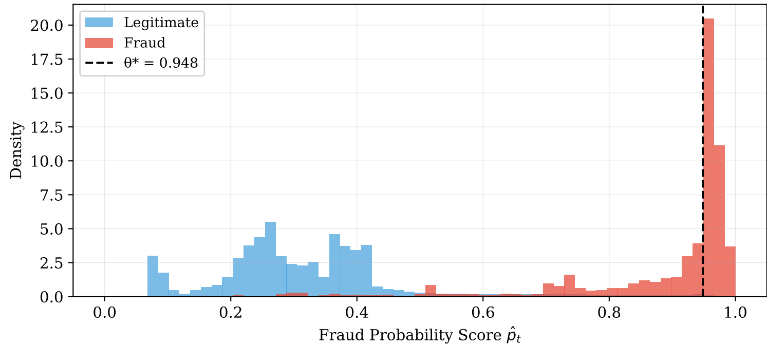
Distribution of Fraud Probability Scores (Test Set)
