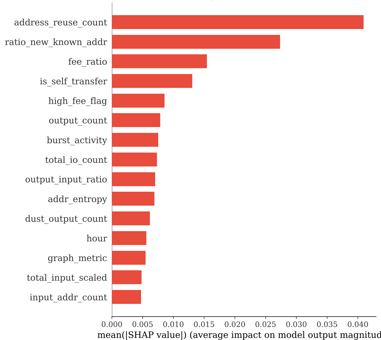
SHAP Feature Importance — GriffinGNN (Test Set)
