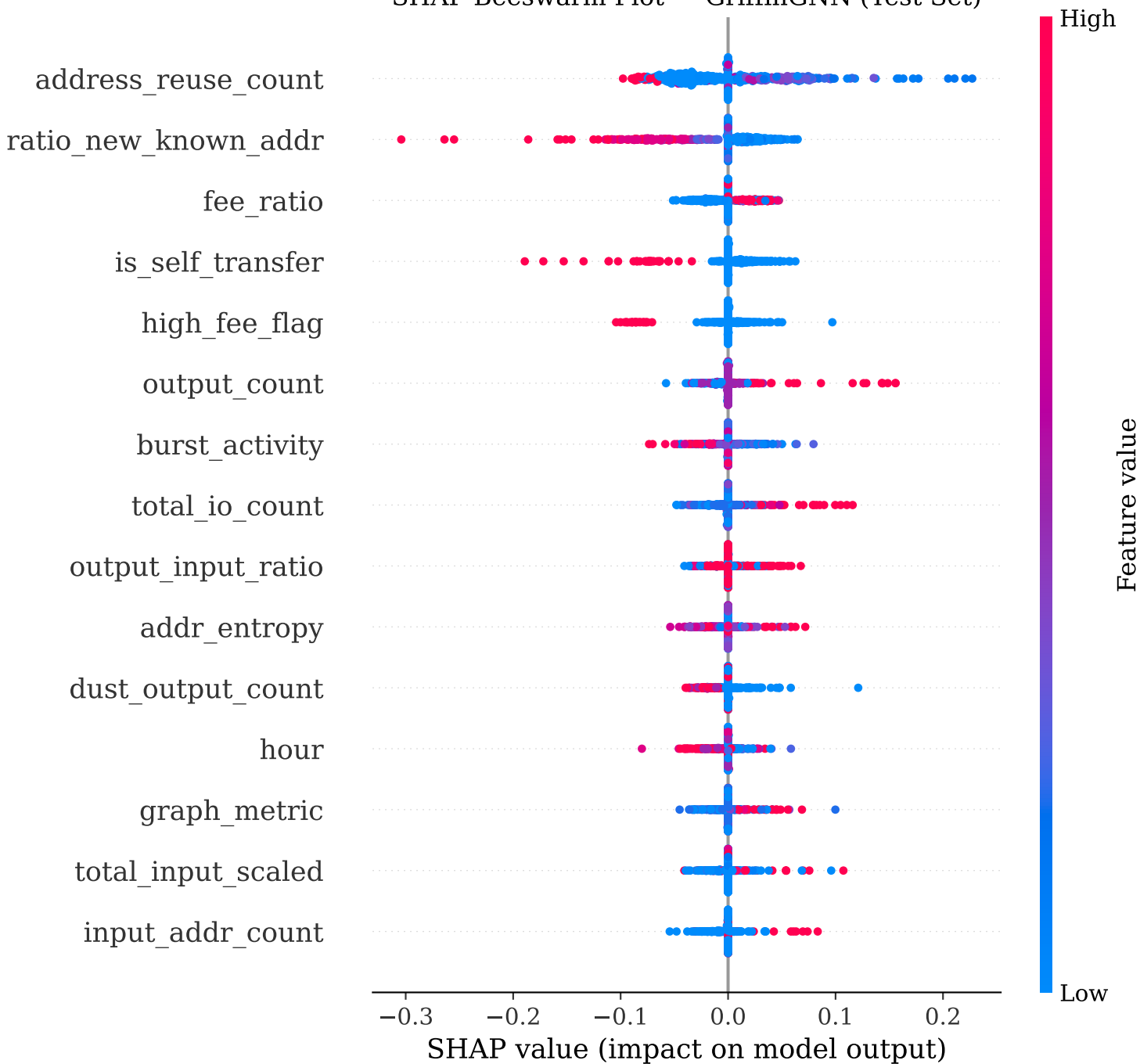
SHAP Beeswarm Plot — GriffinGNN (Test Set)
