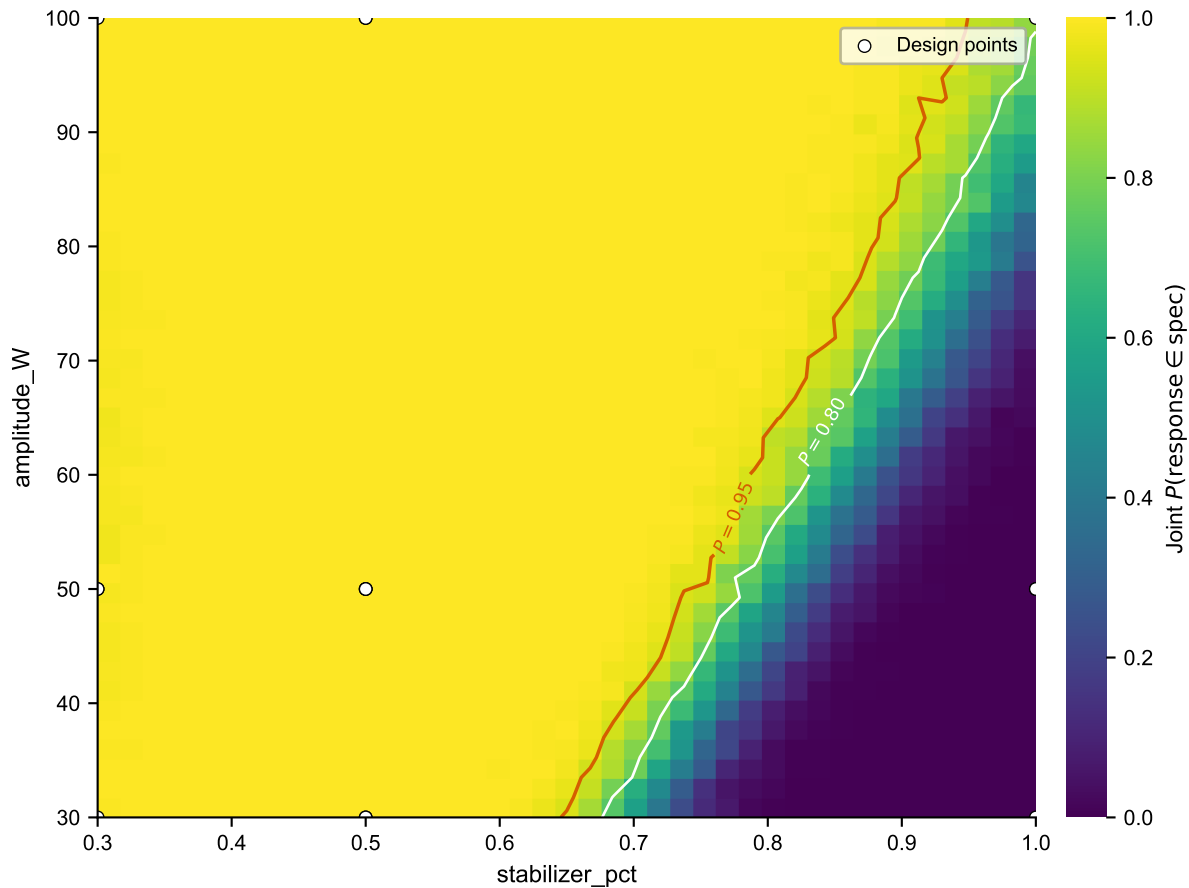
Figure 8. Probabilistic design space - case3_boscolo_2023_BBD_lyo
