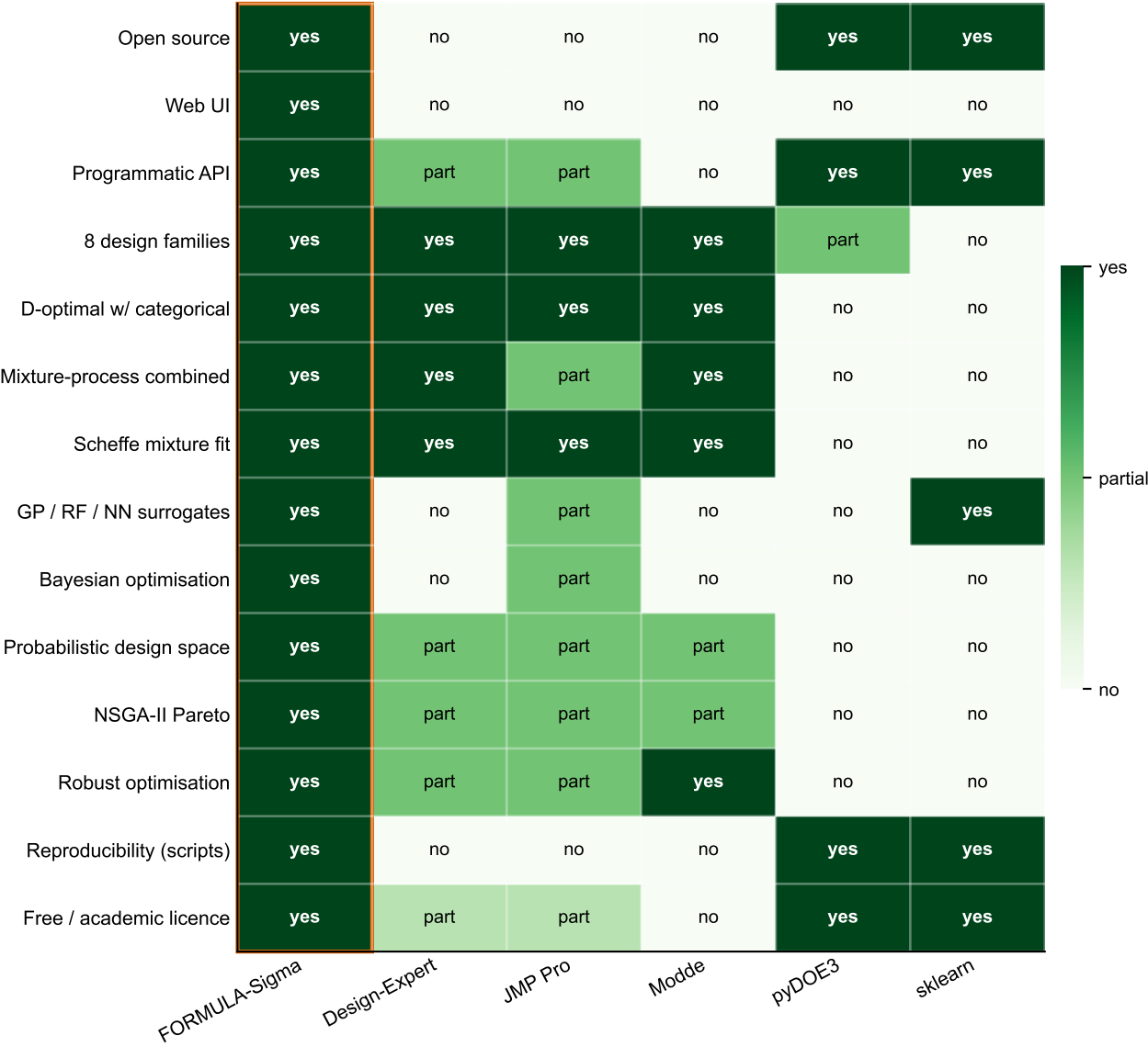
Figure 2. Feature parity: FORMULA-Sigma vs commercial and open competitors
