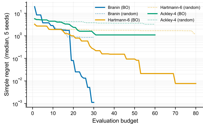
(a) Bayesian optimisation vs random search
