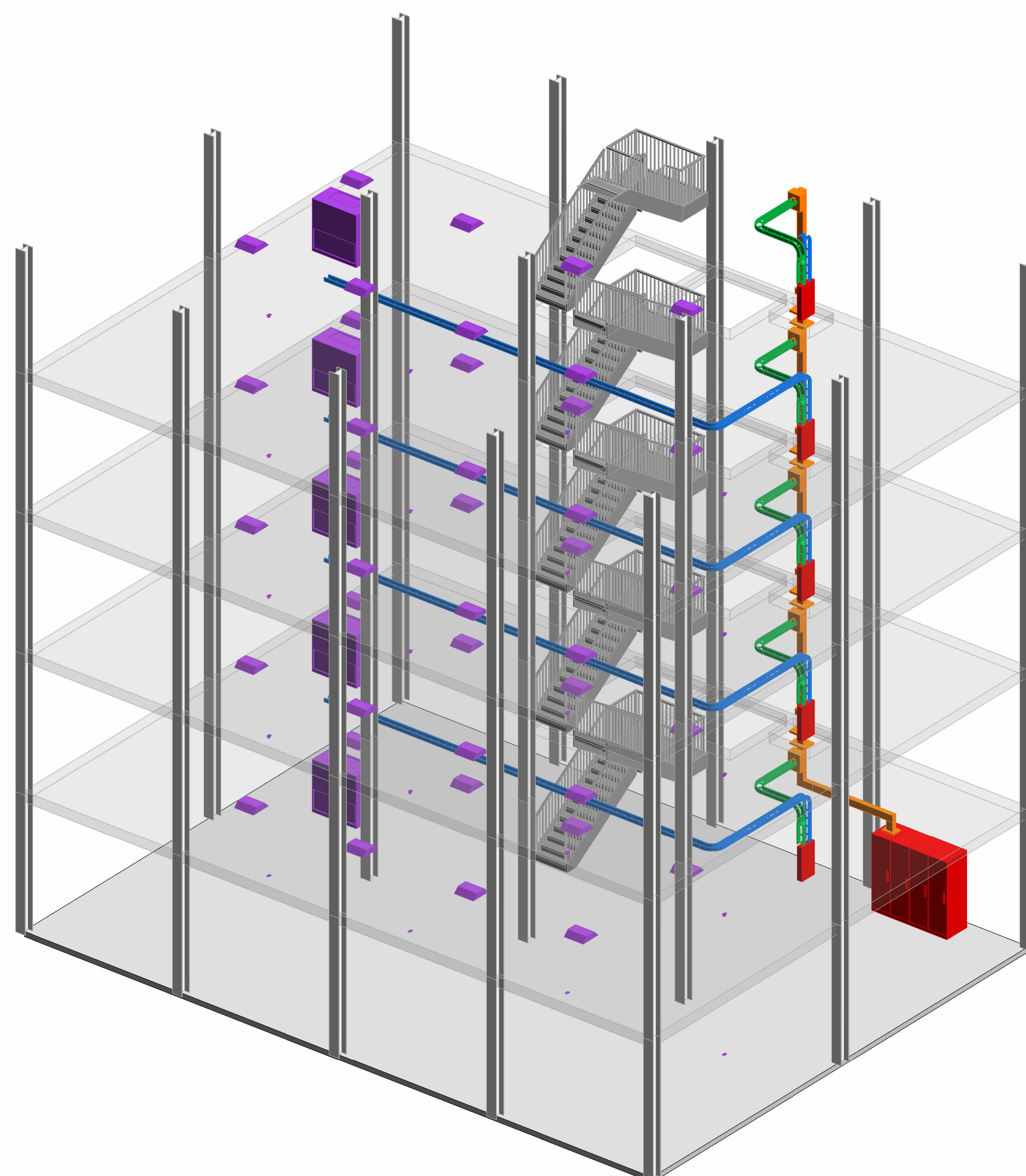
1 3D - Busduct System
