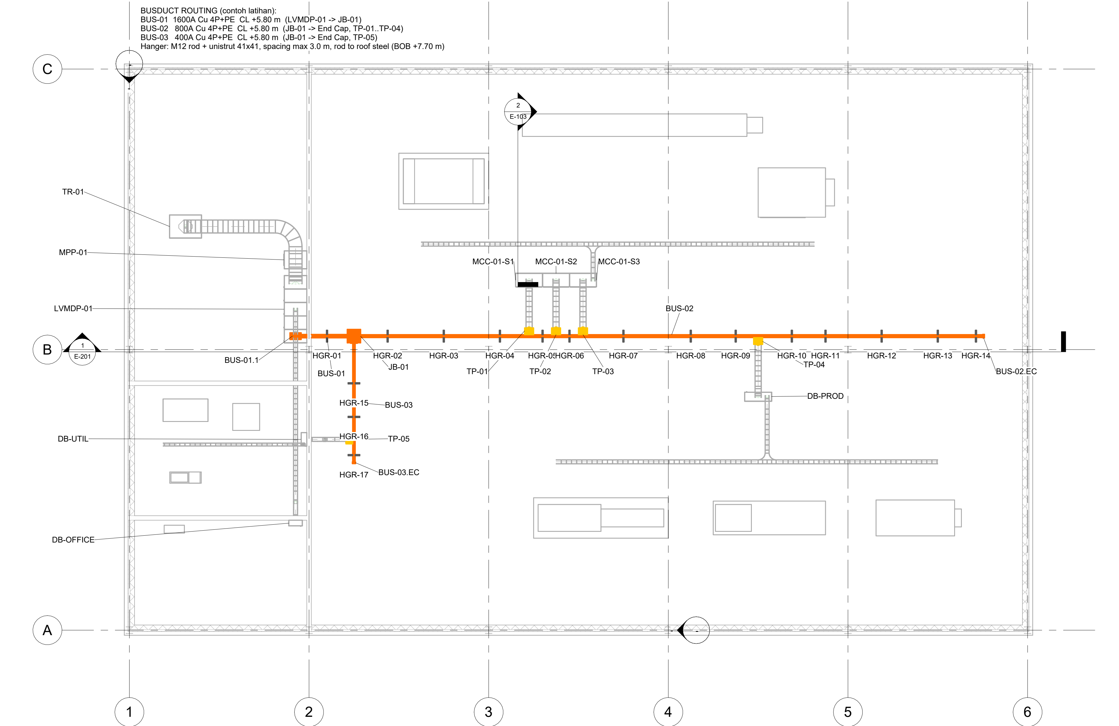
1 EL-02 Busduct Layout Plan 1 : 100
