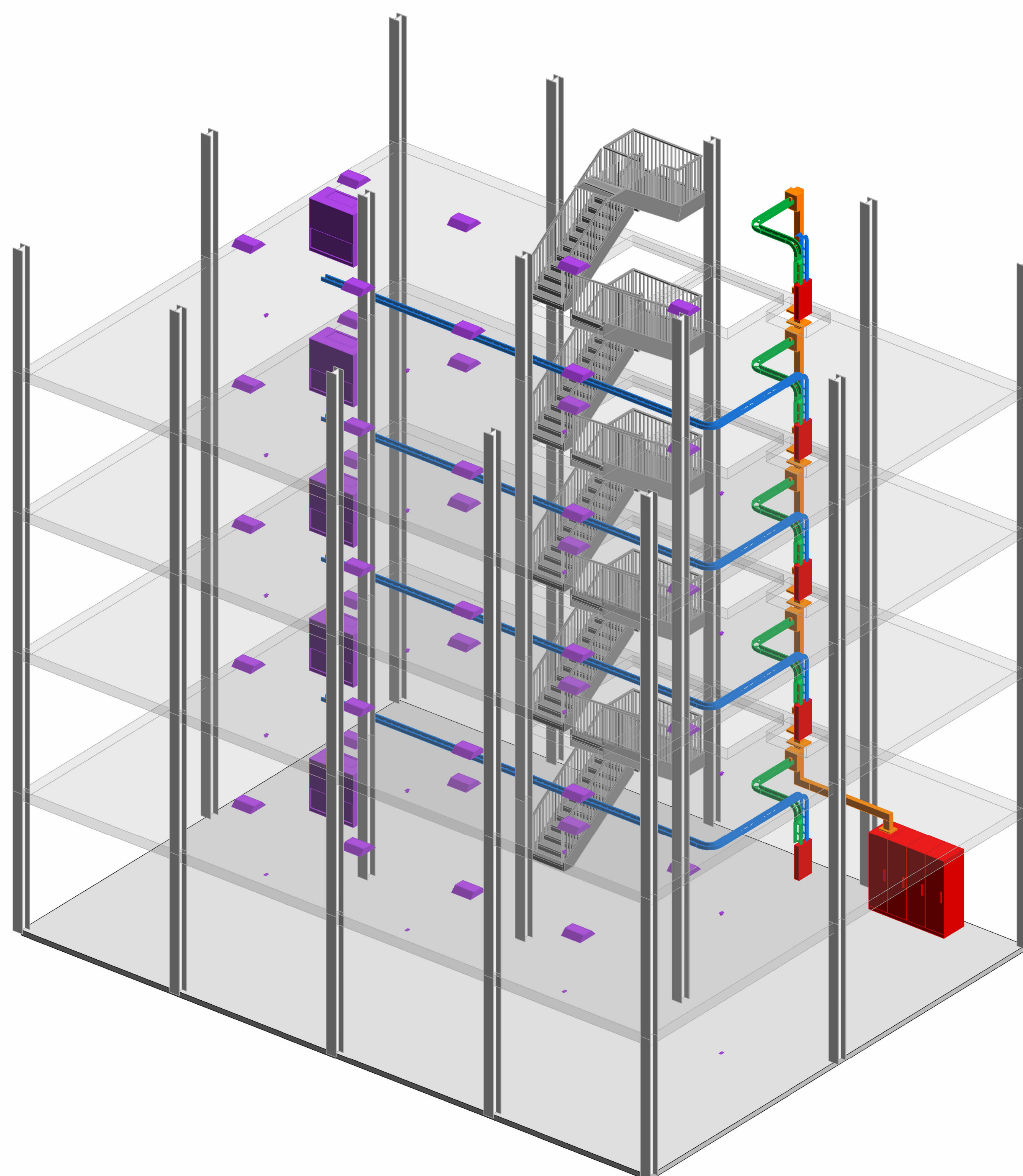
1 3D - Busduct System
