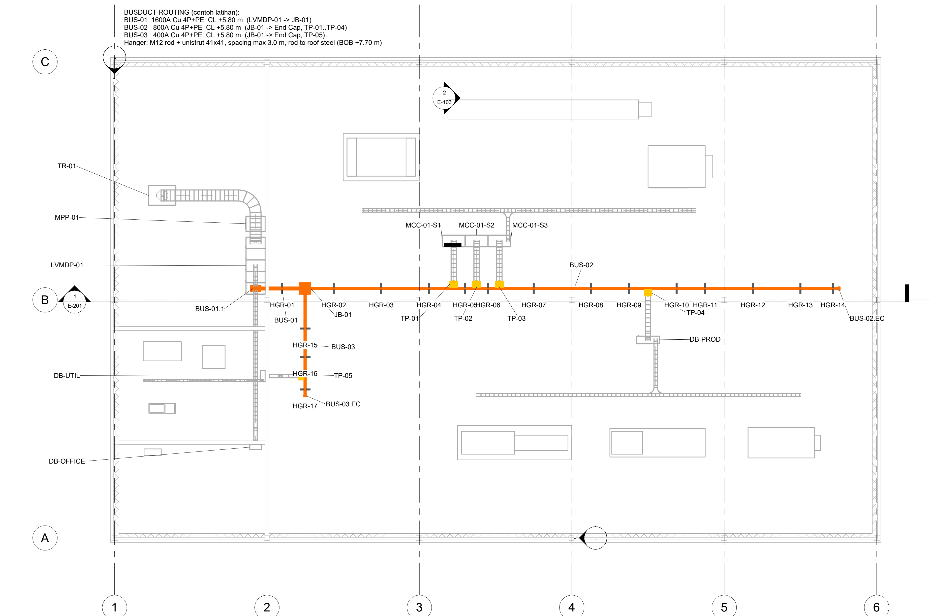
1 EL-02 Busduct Layout Plan 1 : 100
