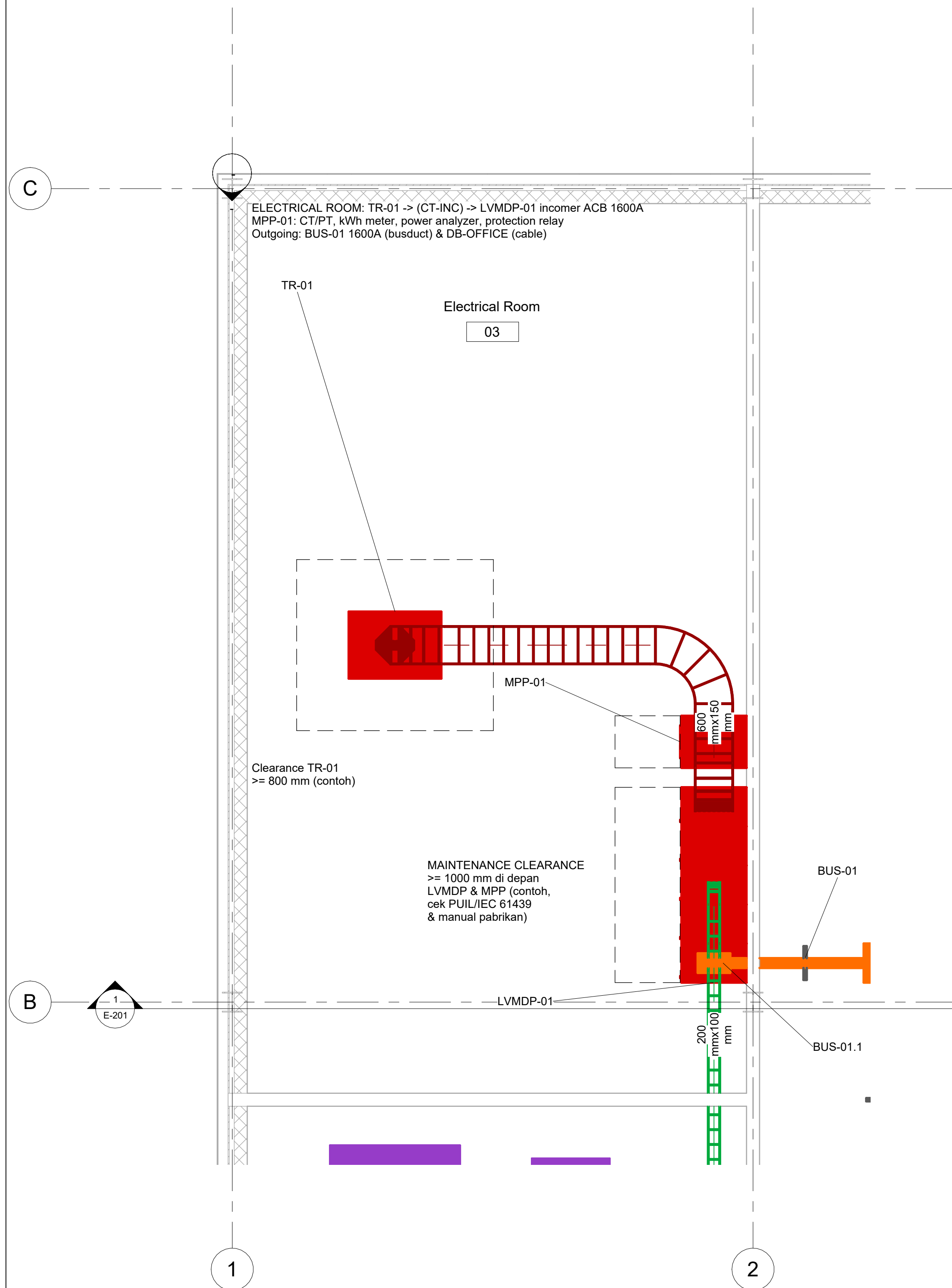
EL-03 Electrical Room Plan
