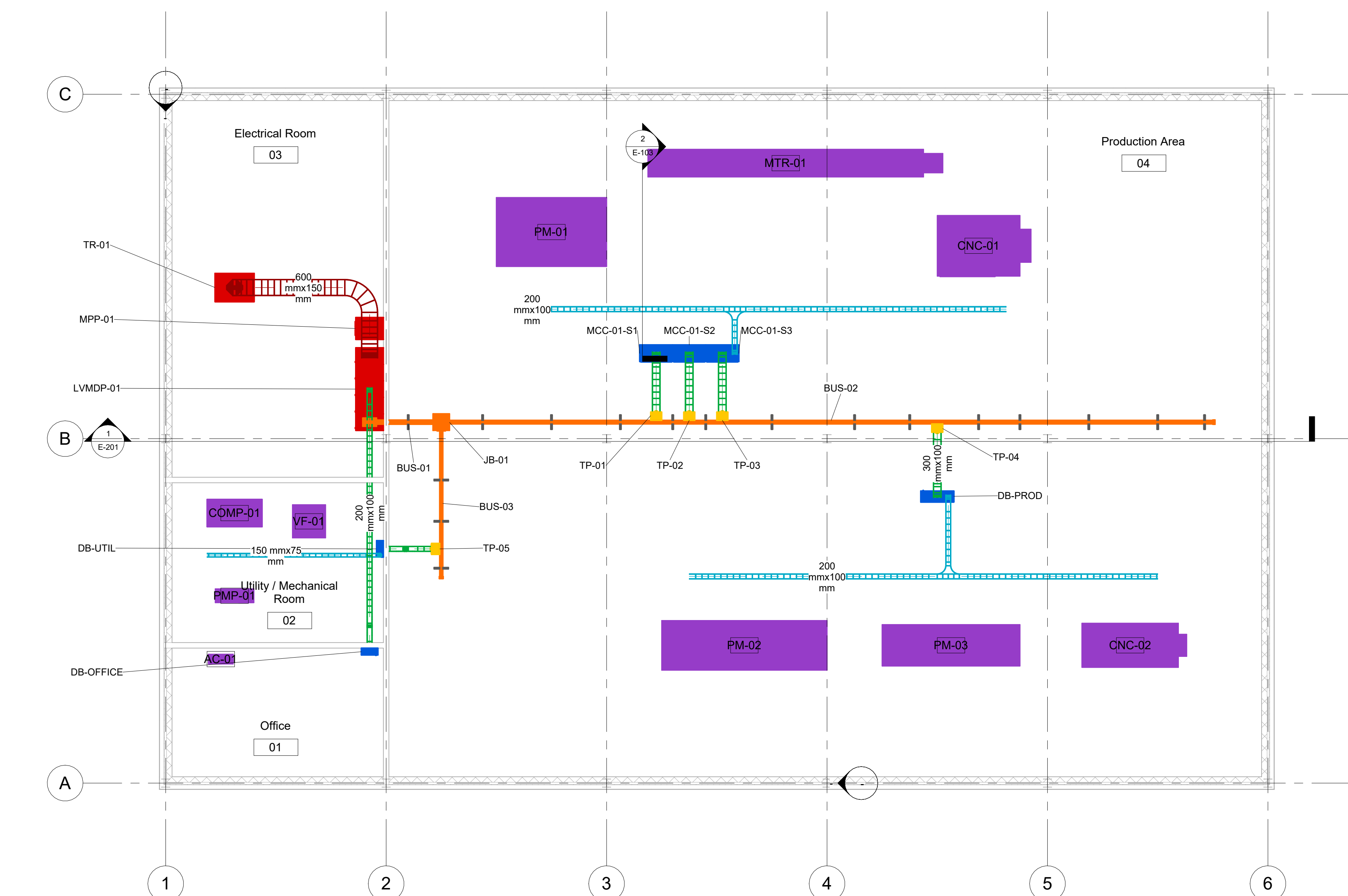
1 EL-01 Electrical Layout Plan 1 : 100
