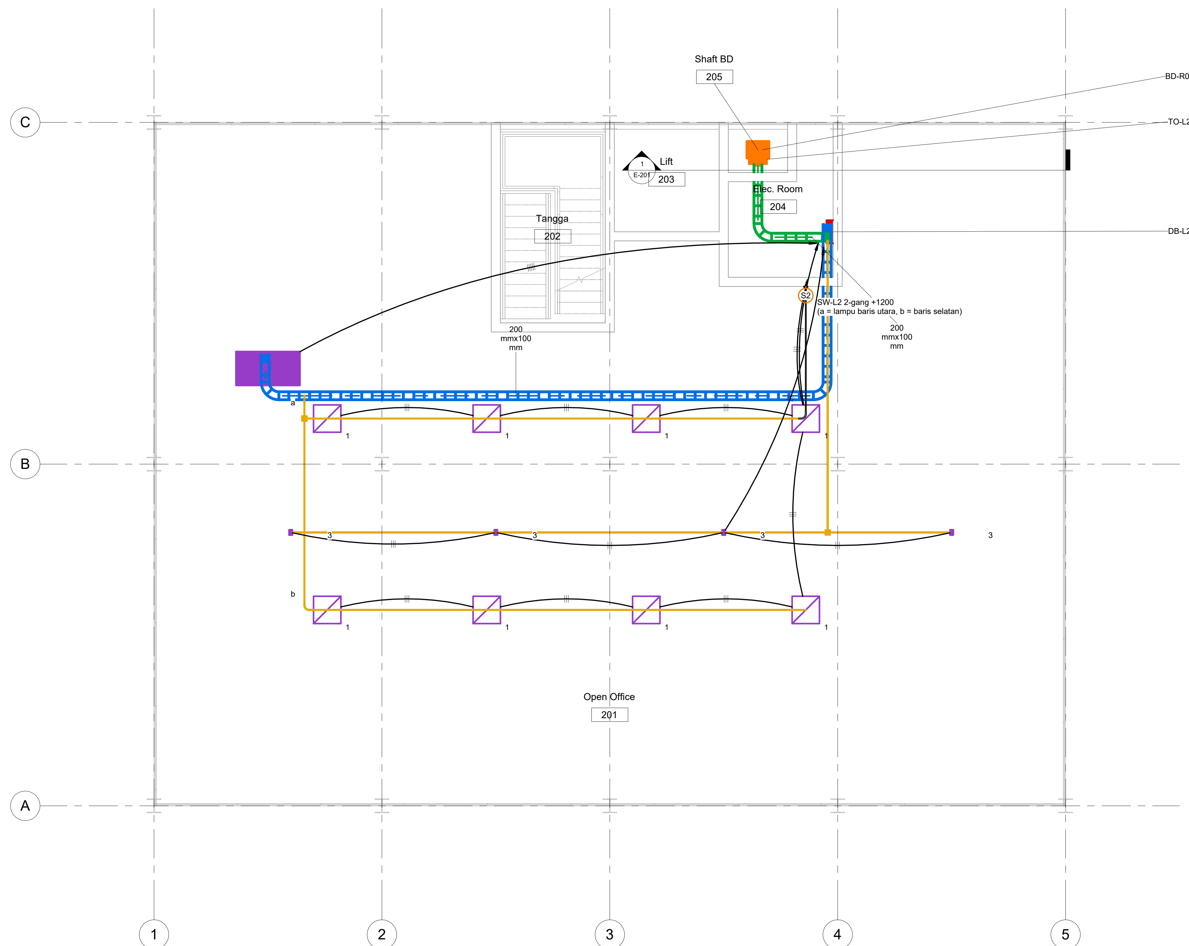
1 E-L2 Denah Tipikal Lantai 2-5 - Busduct & Power 1 : 50
