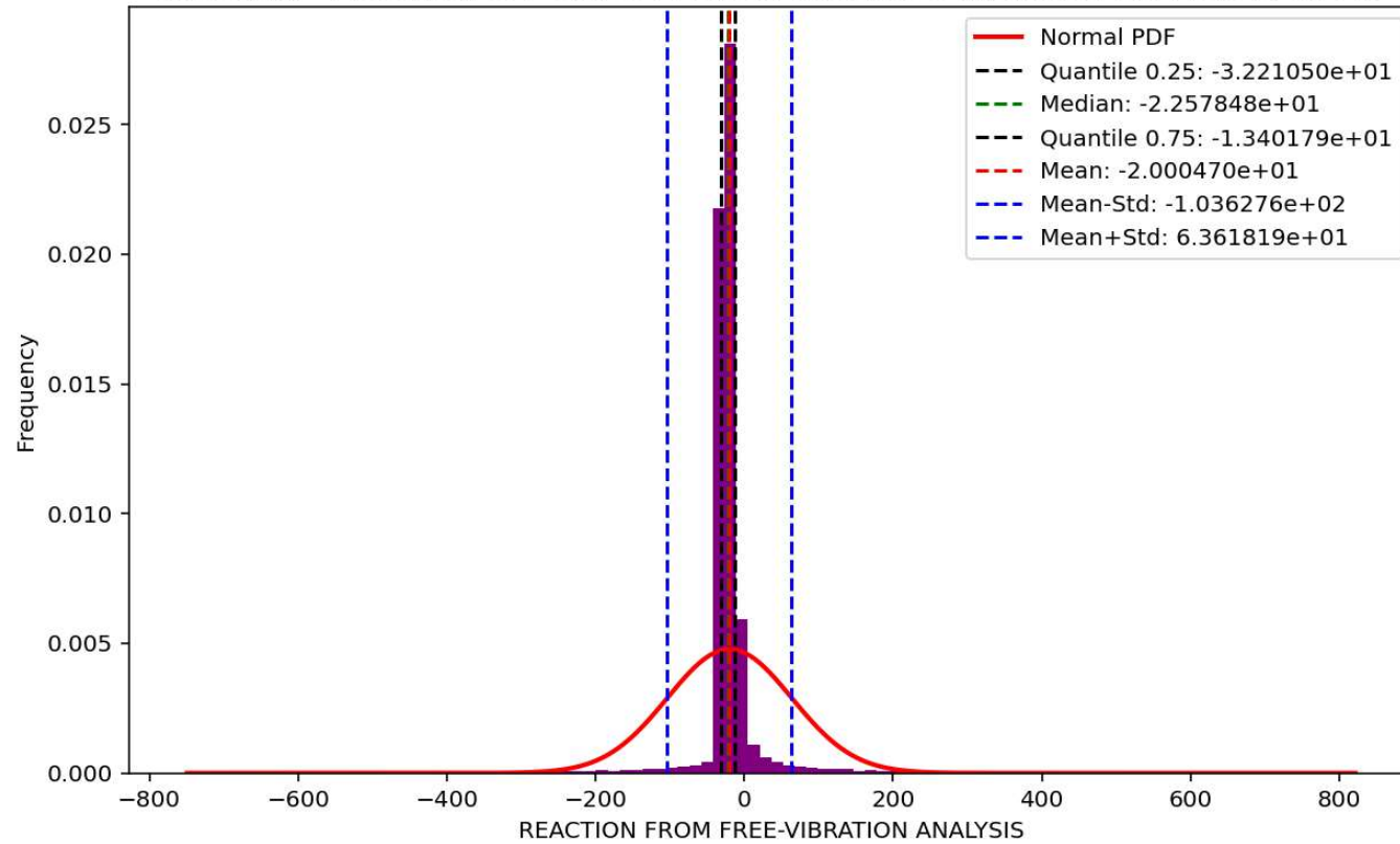
Histogram - Probability of Positive REACTION FROM FREE-VIBRATION ANALYSIS is 8.40 %
